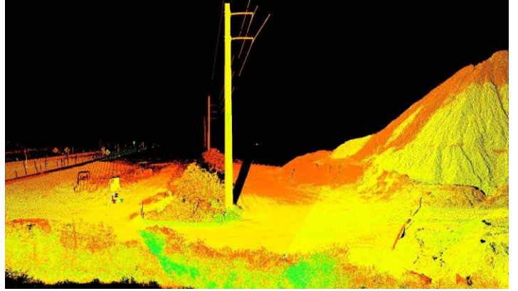
Point Cloud Data Tied to Survey
